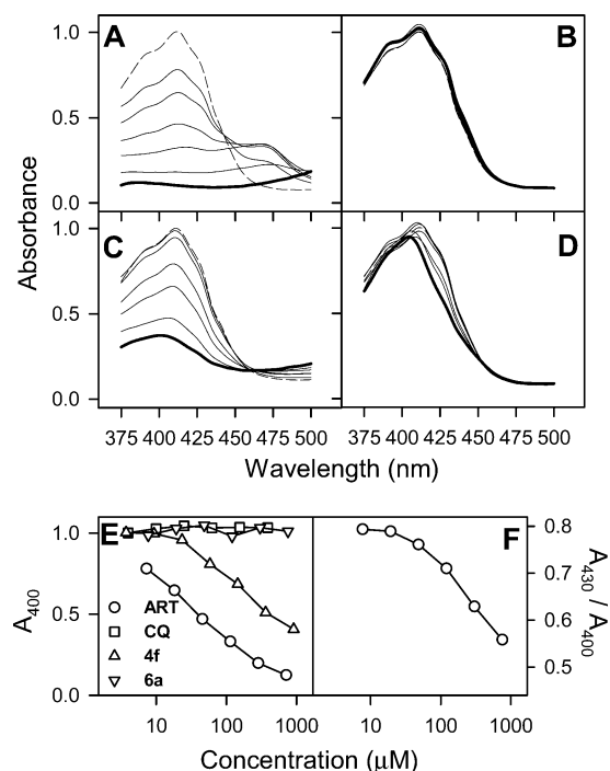
Figure 4. Spectral analysis of the interactions of CQ, artemisinin, and some novel endoperoxides with FP-Fe(II): absorption spectra of 30 \mu\text{M} FP-Fe(II) in the presence of (A) artemisinin, (B) CQ, (C) 4f , and (D) 6a under reducing conditions. The spectra in the presence of the highest concentration of compound (710, 390, 900, and 750 \mu\text{M} compound, respectively) are represented by the thick curves, whereas the spectra for FP-Fe(II) alone are the dashed curves. The dilution factor for intermediate concentrations is 2.5. The spectra are normalized to that of FP in the absence of compound and are shown at wavelengths above 375 nm because of the large absorbance of the dithionite ion at shorter wavelengths. The dose dependence of the loss of the Soret absorption at 400 nm is shown in (E). In some cases, compounds induce a change in the structure of the Soret band rather than a loss of absorbance. The absorbance ratio at 430 and 400 nm ( A_{430}/A_{400} ) indicates changes to the structure of the Soret band. The dose dependence of this parameter for 6a is shown in (F).
